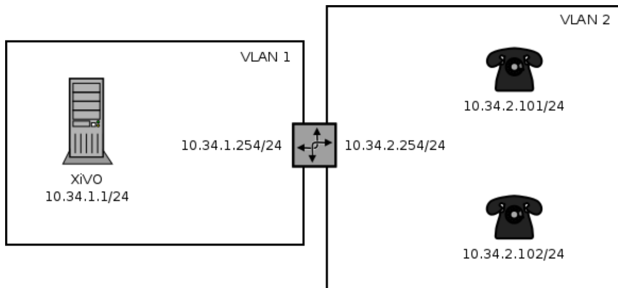
Fig. 1: Phones behind a NAT
